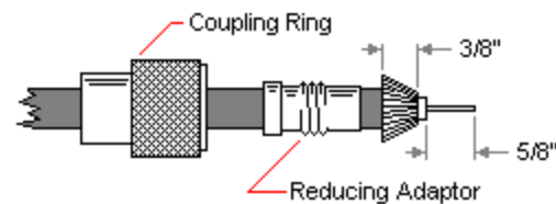
PL259 (With adapter)
